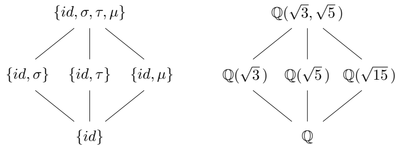
Figure 23.1. G(\mathbb{Q}(\sqrt{3}, \sqrt{5})/\mathbb{Q})
